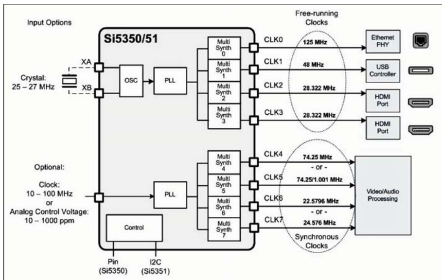
Figure 4 · Silicon Labs Si5350/51 programmable general-purpose clock IC.
