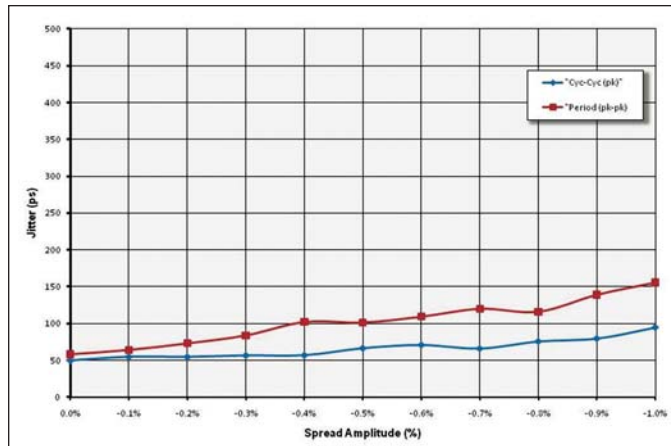
Figure 3 · SSCG also minimizes period and cycle-to-cycle jitter.
