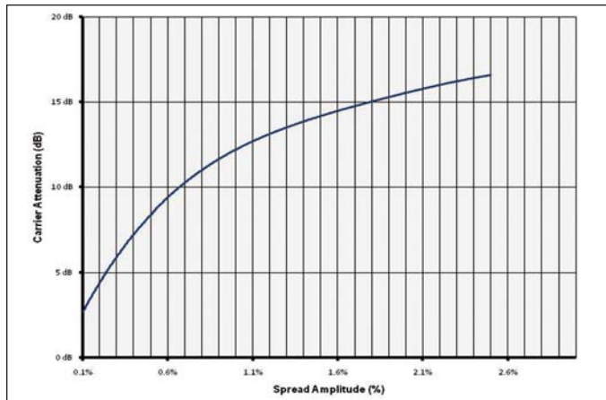
Figure 2 · Spread spectrum clock generation (SSCG) reduces EMI at any single frequency.
