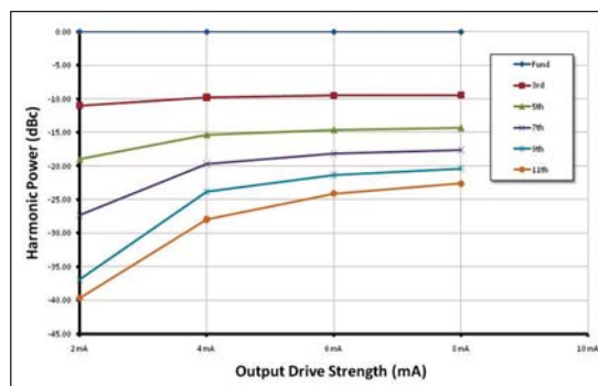
Figure 1 . Relative carrier and harmonic power vs. output drive strength at 10 MHz (Example: Silicon Labs Si5350/51 Clock IC).
